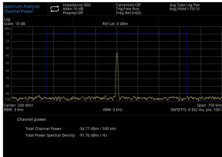
Figure 5-1 Channel Power
