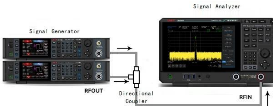
Figure 3-4 Instrument Setting for Acquire Signal from Two Channel
