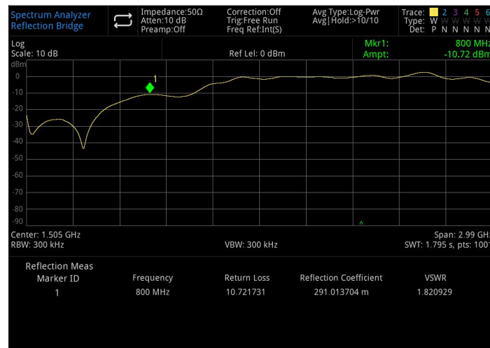
Figure 5-9: Reflection Meas
