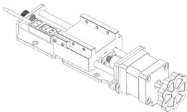
Electric lifting module X1
