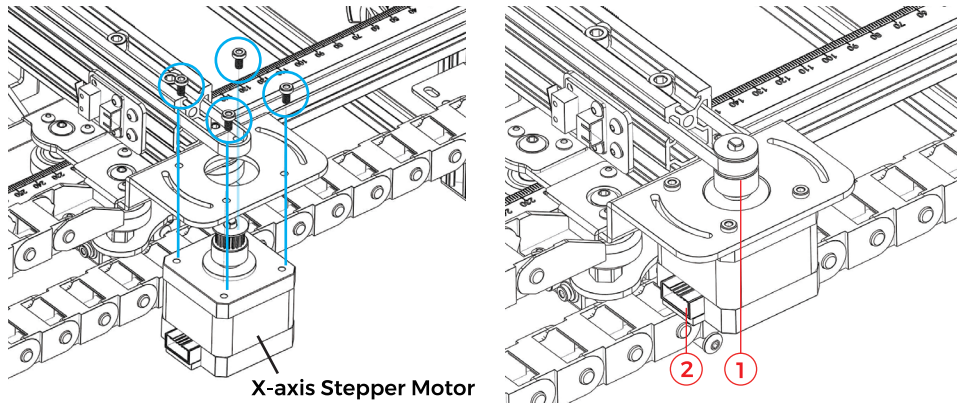
X-axis Stepper Motor
