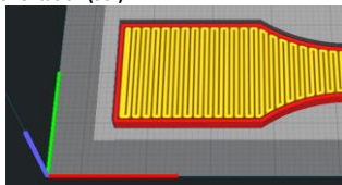
X-Y-orientation (90°)
