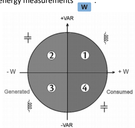
Figure 17-3: Four-quadrant diagram for power and energy
