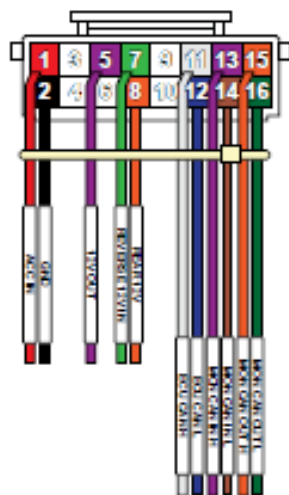
POWER/CAN CABLE
