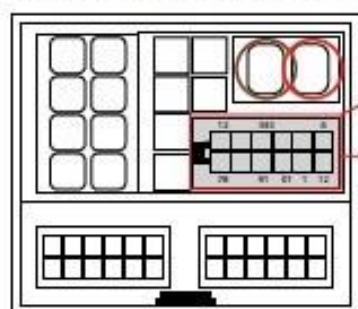
MIB2 Head Unit Main Harness
