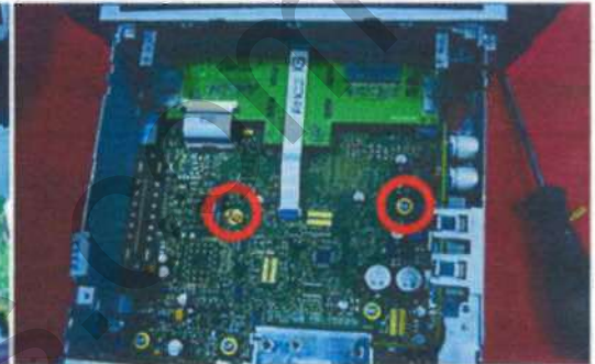
7. Remove the screws and install the copper posts
