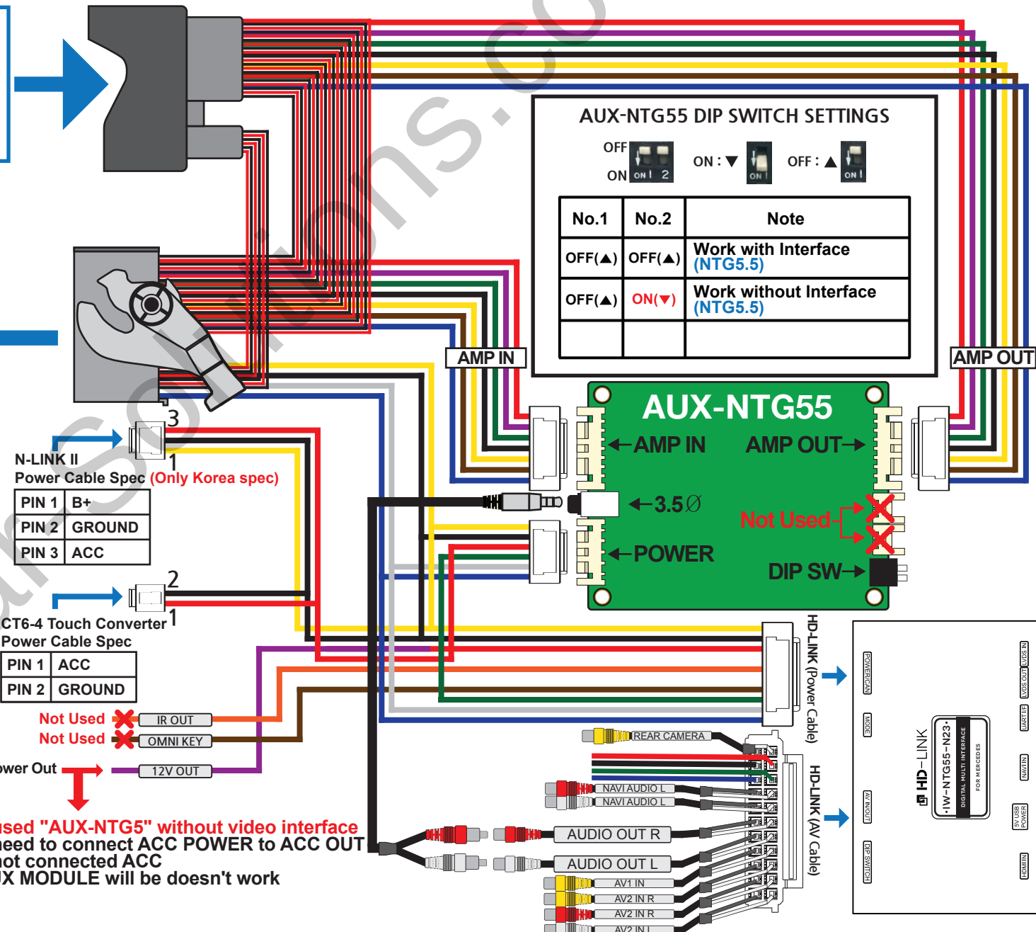
AUX-NTG55 HEAD UNIT MAIN CONNECTOR
