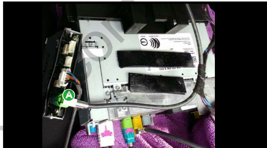
2. PLEASE USE THE PULLED OUT OEM LVDS CABLE (A) CONNECT WITH LVDS IN OF INTERFACE.
