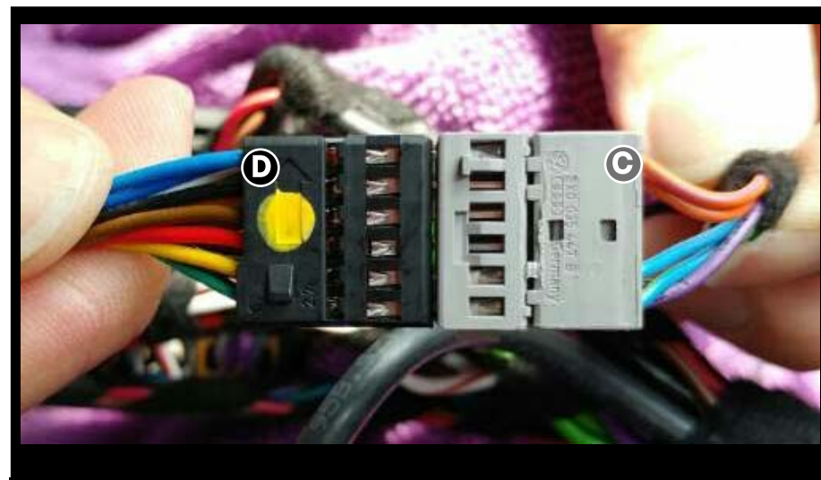
4. PLEASE USE REMOVED OEM CONNECTOR (C) CONNECT WITH (D) AS PICTURE SHOWED.
