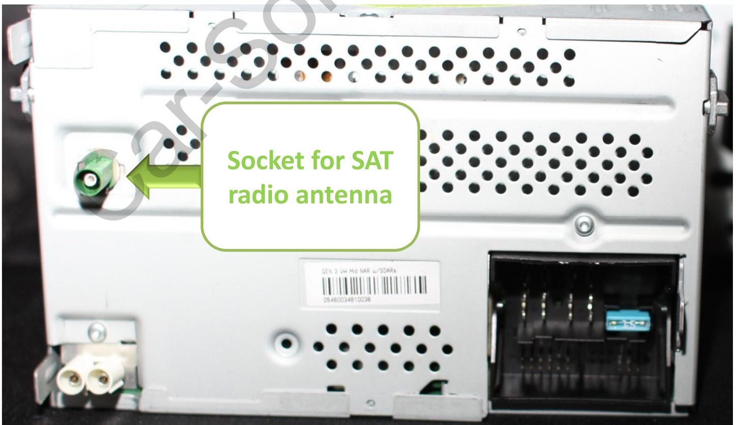
Rear side of RCD510 Delphi monitor with satellite radio function («SAT»)
