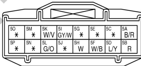
OEM navigation unit connectors numbering from wires side
